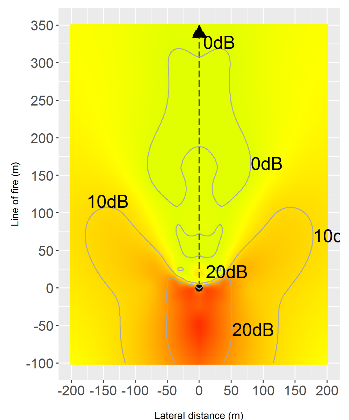
Fig 3. Peak noise reduction in 10dB steps (see contours) highlighting the reduction each side and to the rear of the shooter. The arrow indicates the line of fire.
